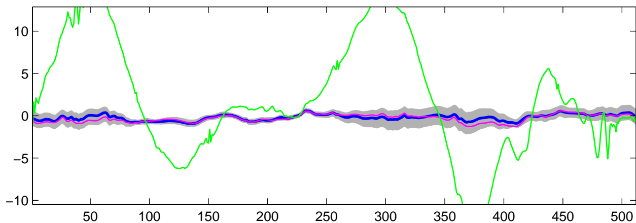
Estimated C_2(t) using R-WFMM: t_1 data, run 3
