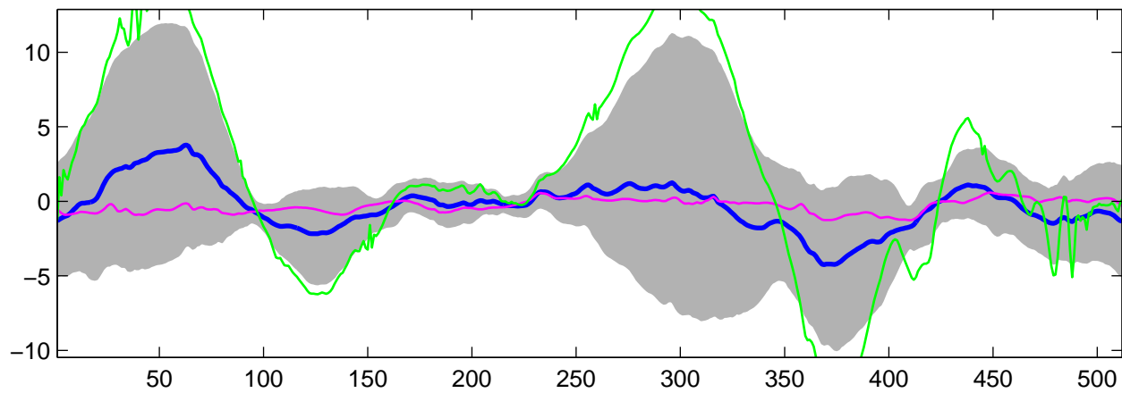
Estimated C_2(t) using G-WFMM: t_1 data, run 3
