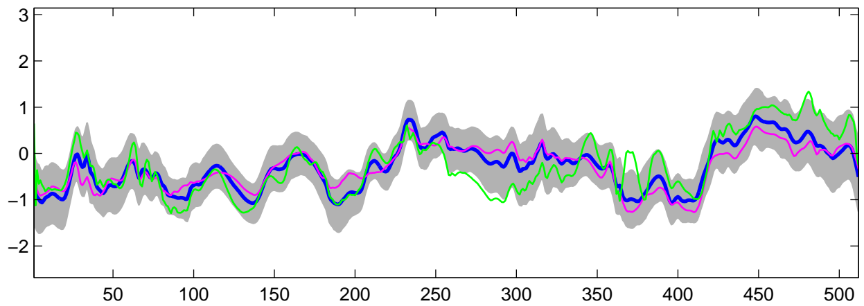
Estimated C_2(t) using R-WFMM: t_2 data, run 3
