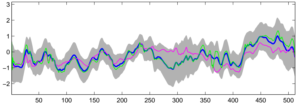
Estimated C_2(t) using G-WFMM: t_2 data, run 3
