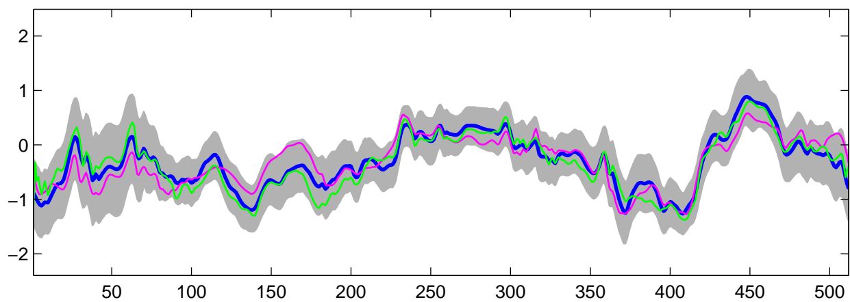
Estimated C_2(t) using R-WFMM: t_3 data, run 3
