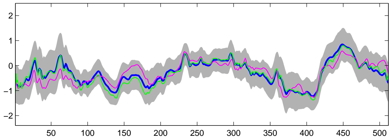
Estimated C_2(t) using G-WFMM: t_3 data, run 3
