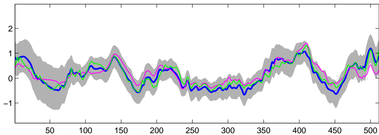
Estimated C_3(t) using R-WFMM: t_3 data, run 3
