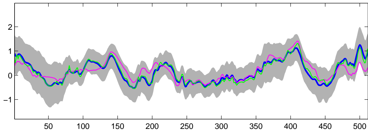
Estimated C_3(t) using G-WFMM: t_3 data, run 3
