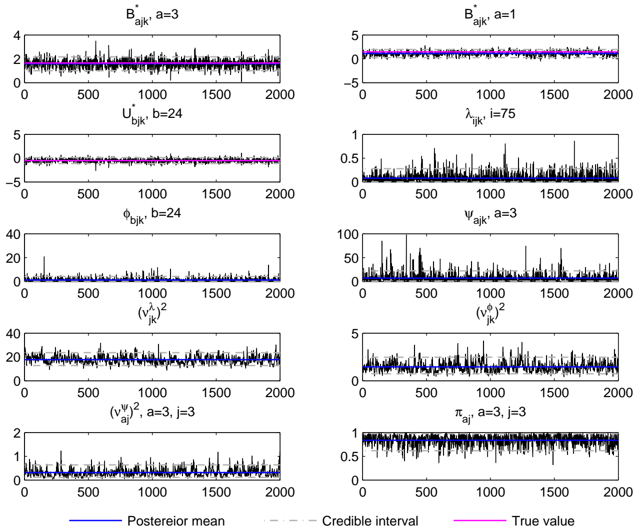
Trace plot, j=3, k=4 , DE data, simulation run 3
