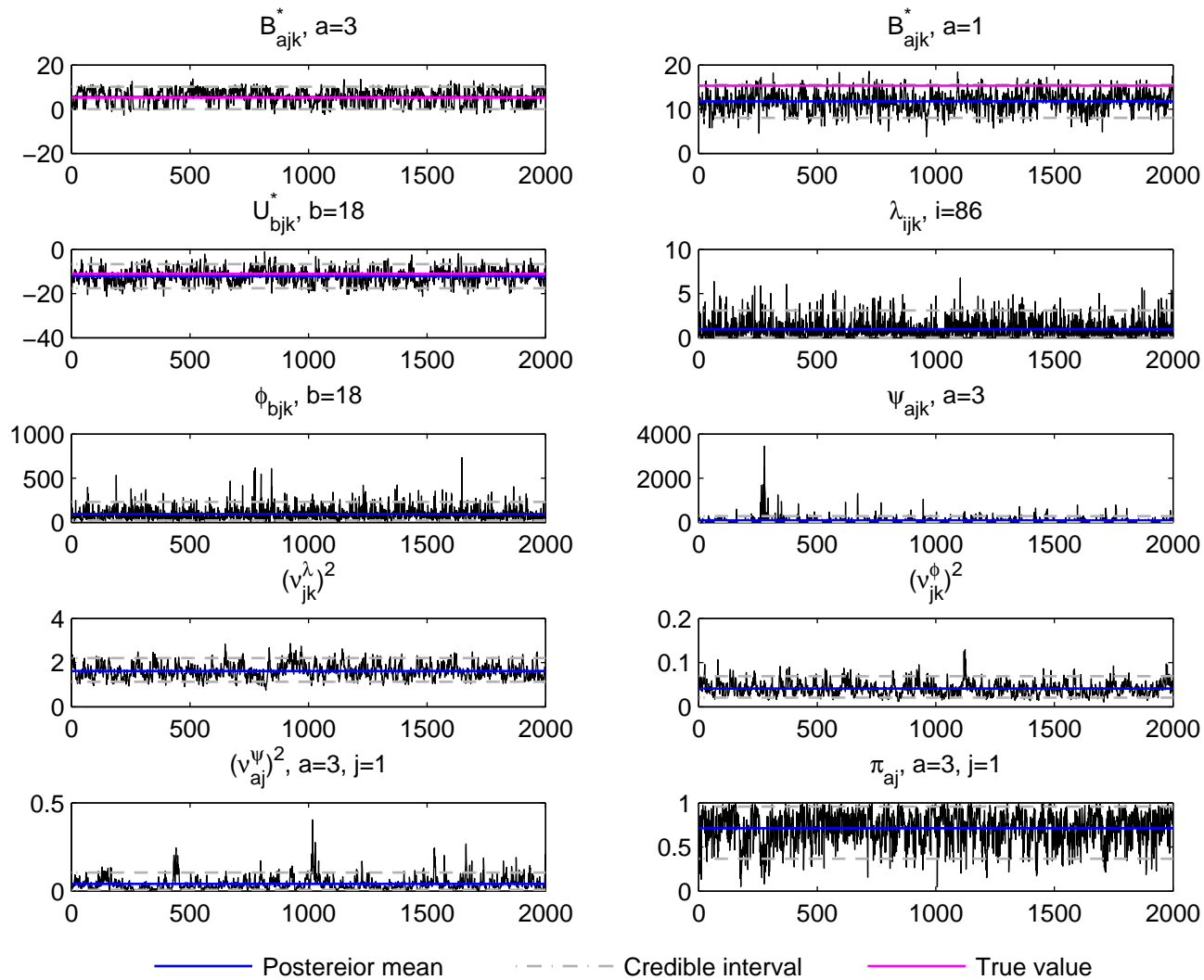
Trace plot, j=1, k=2 , Normal data, simulation run 3
