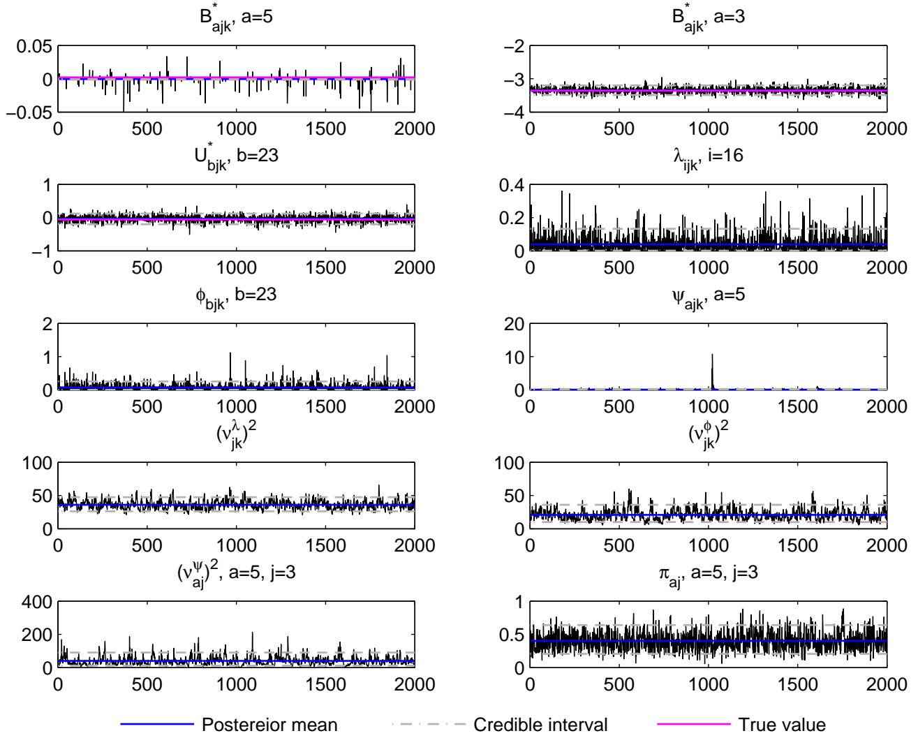
Trace plot, j=3, k=10, t_1 data, simulation run 3
