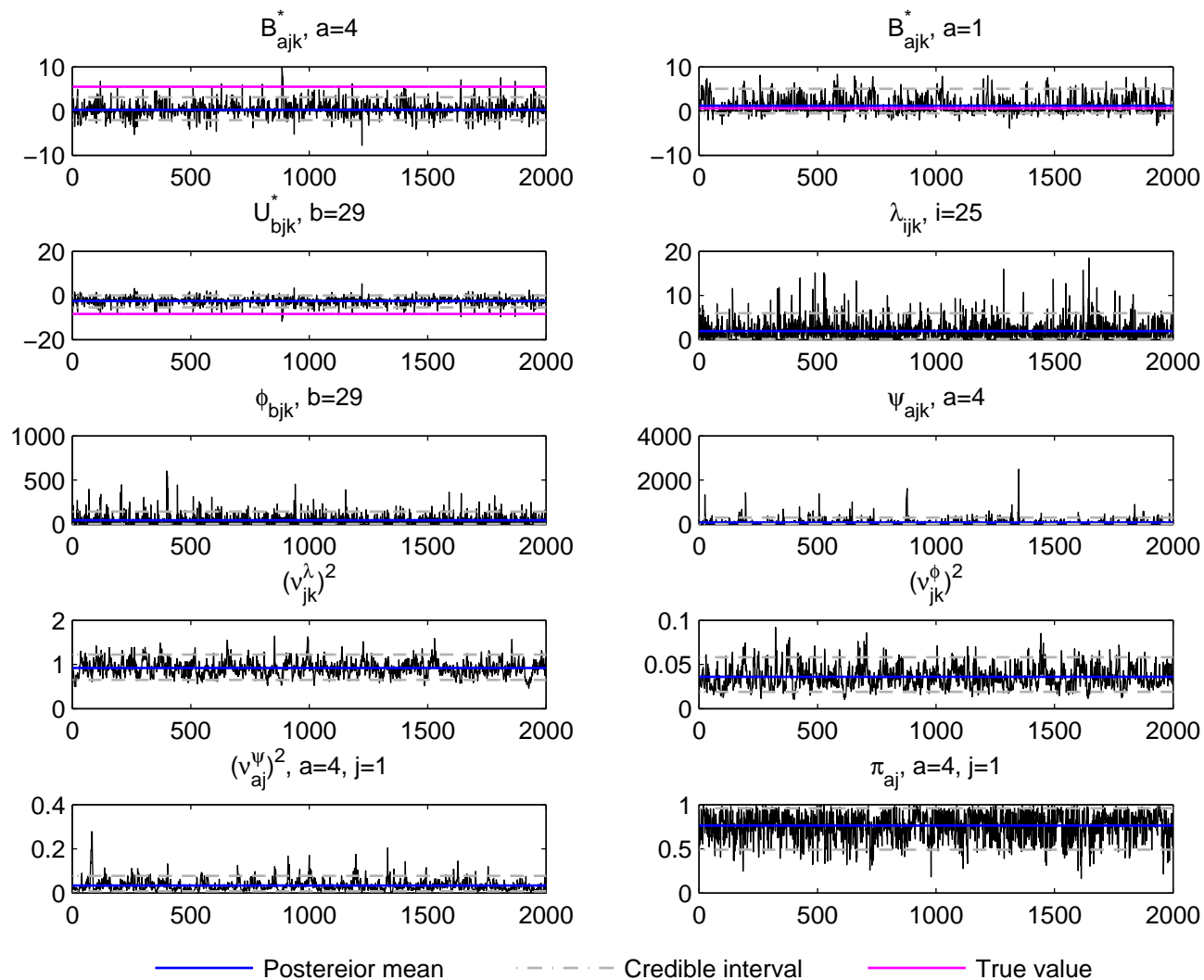
Trace plot, j=1, k=7 , Normal data, simulation run 3
