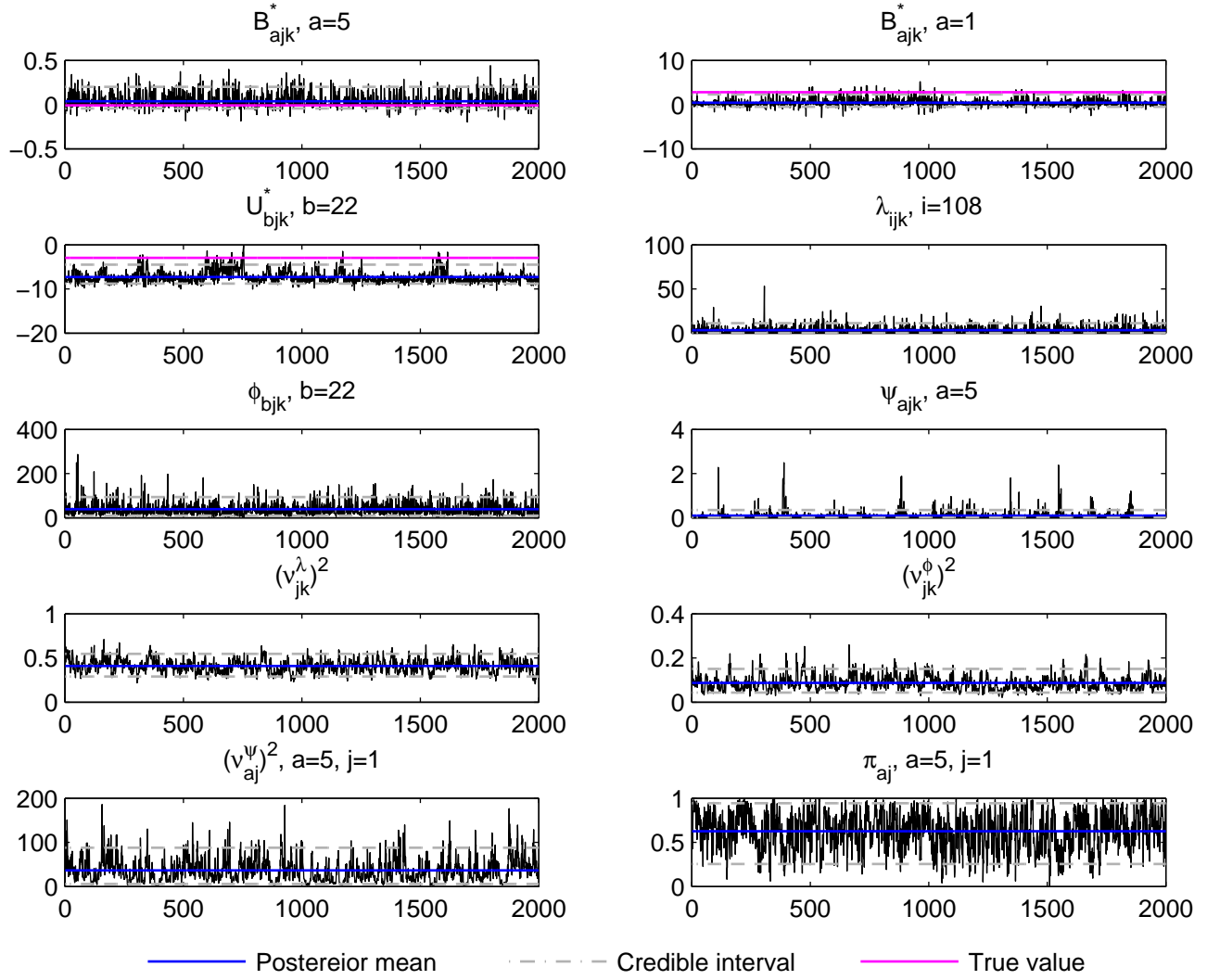
Trace plot, j=1, k=3, t_i data, simulation run 3
