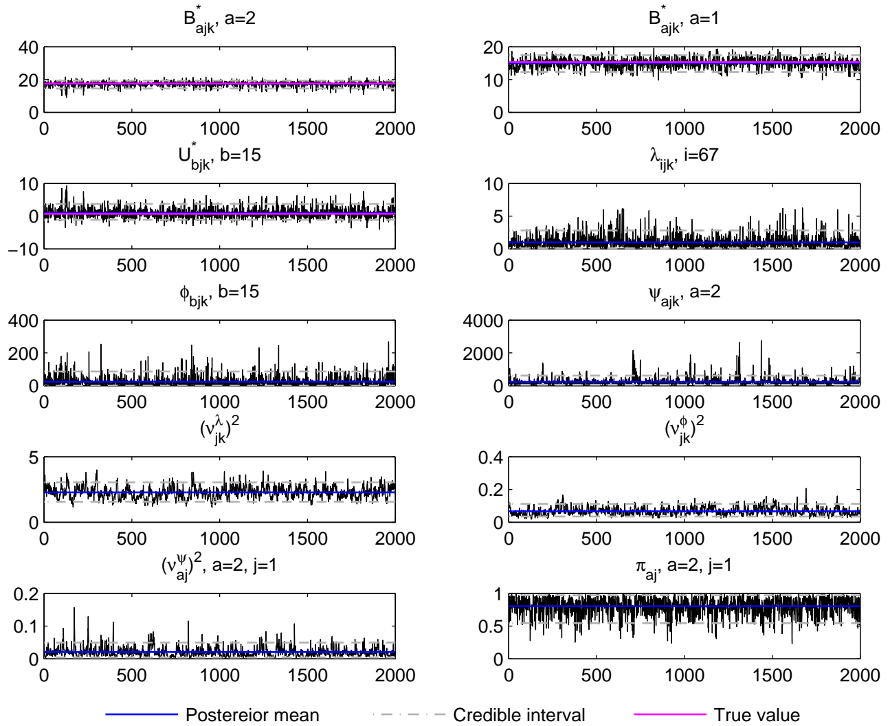
Trace plot, j=1, k=2, t_3 data, simulation run 3
