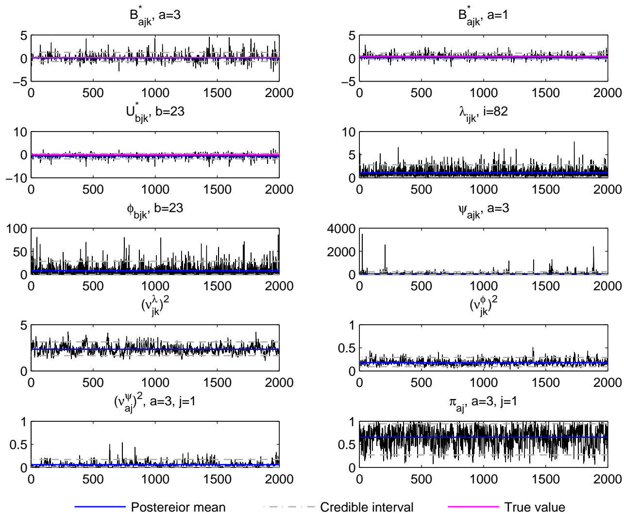
Trace plot, j=1, k=6 , DE data, simulation run 3
