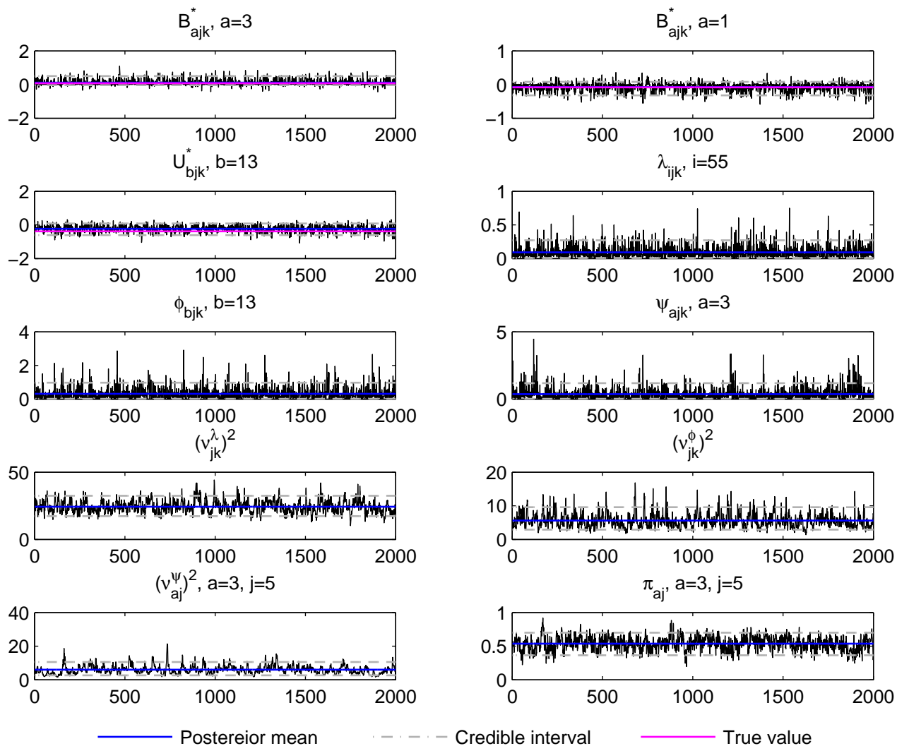
Trace plot, j=5, k=1 , Normal data, simulation run 3
