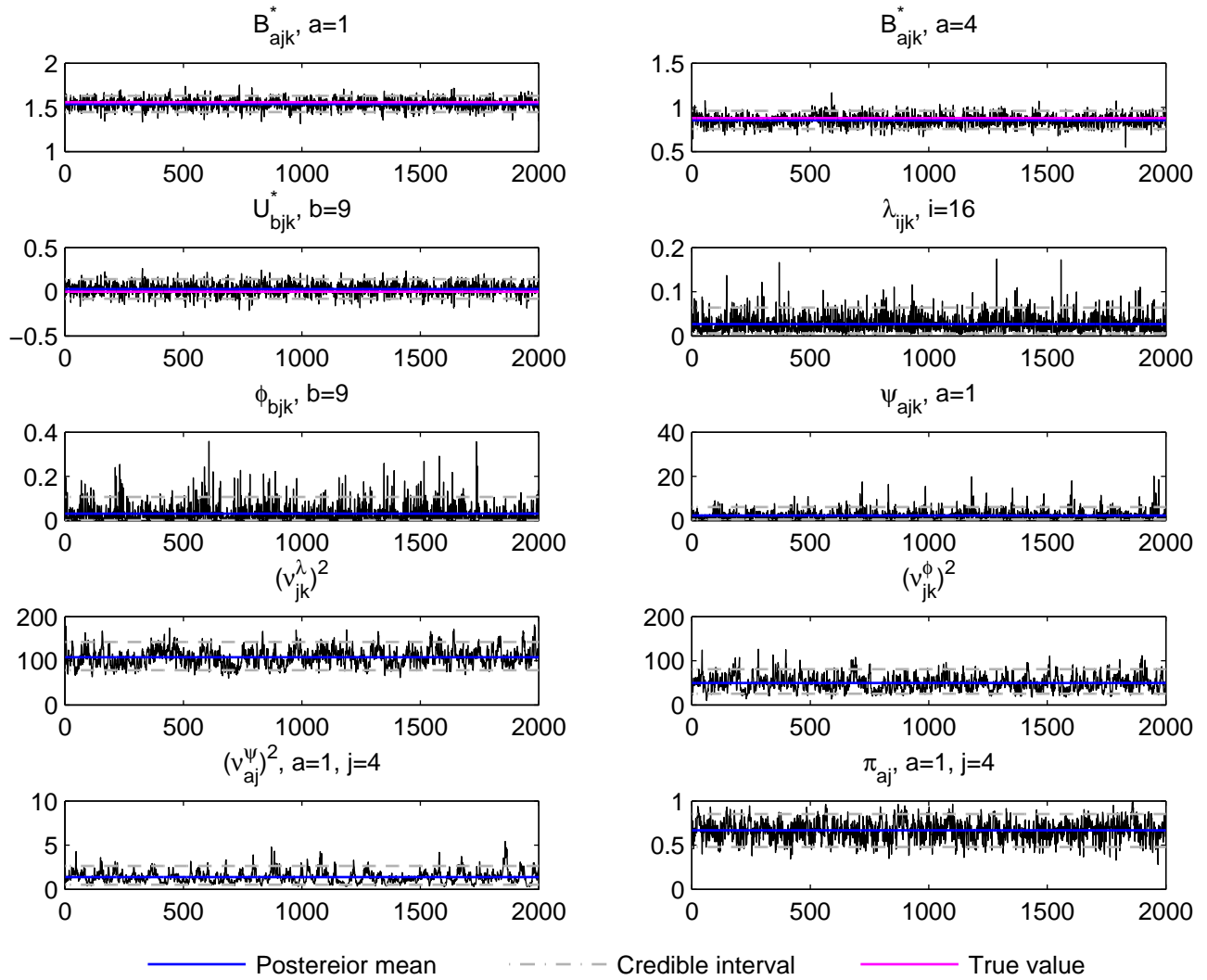
Trace plot, j=4, k=3, t_i data, simulation run 3
