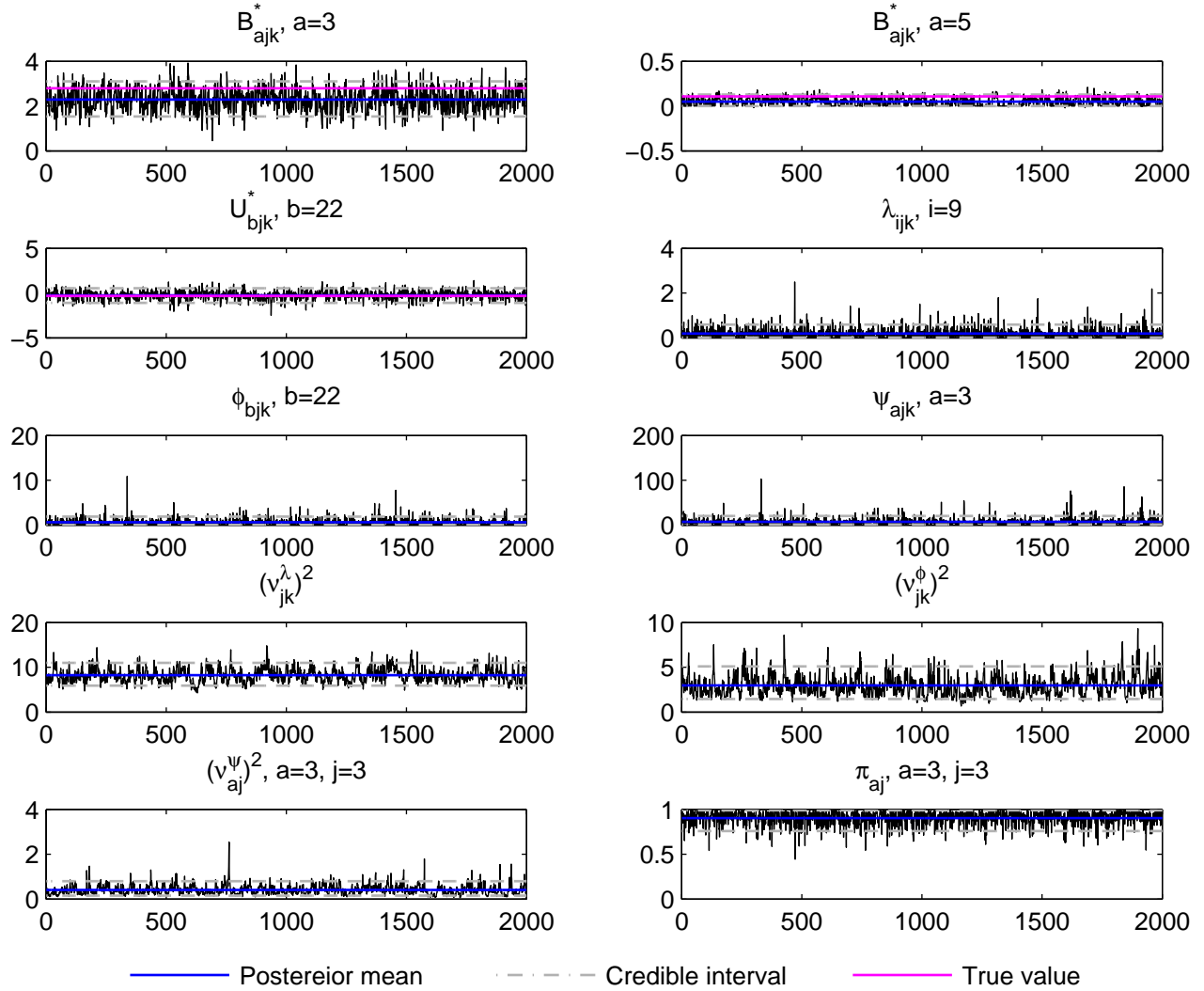
Trace plot, j=3, k=5, t_3 data, simulation run 3
