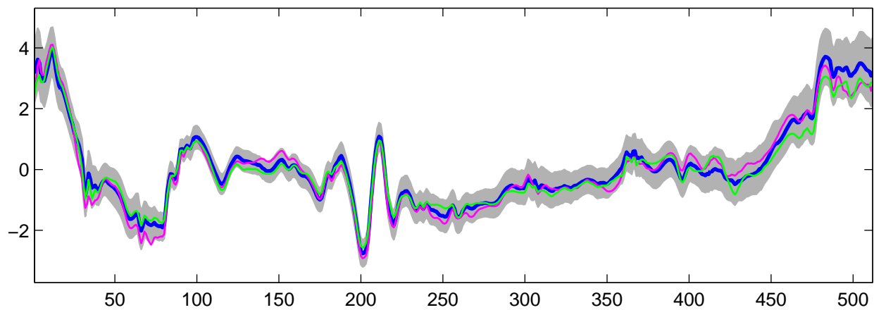
Estimated U_{10}(t) using R-WFMM: DE data, run 3
