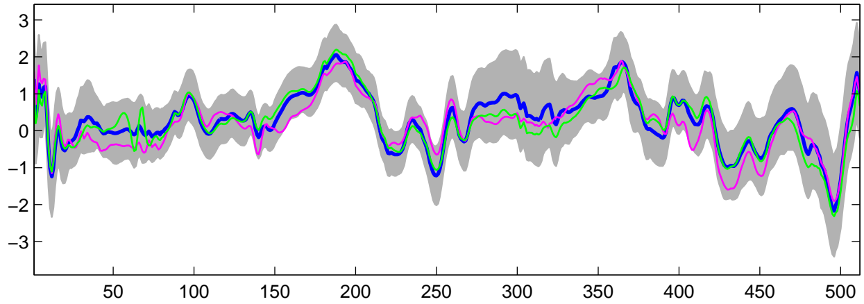
Estimated U_{10}(t) using G-WFMM: t_2 data, run 3
