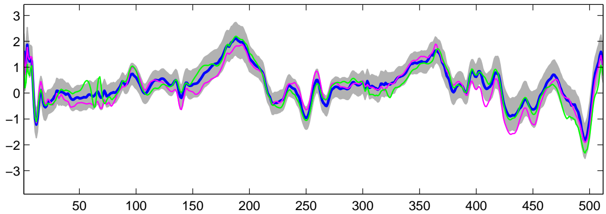
Estimated U_{10}(t) using R-WFMM: t_2 data, run 3
