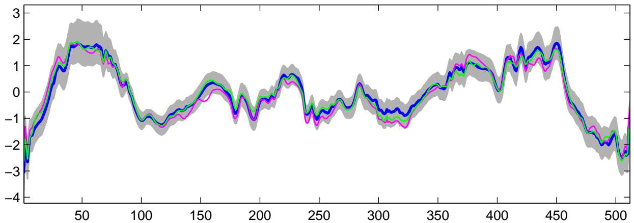
Estimated U_{10}(t) using R-WFMM: t_3 data, run 3
