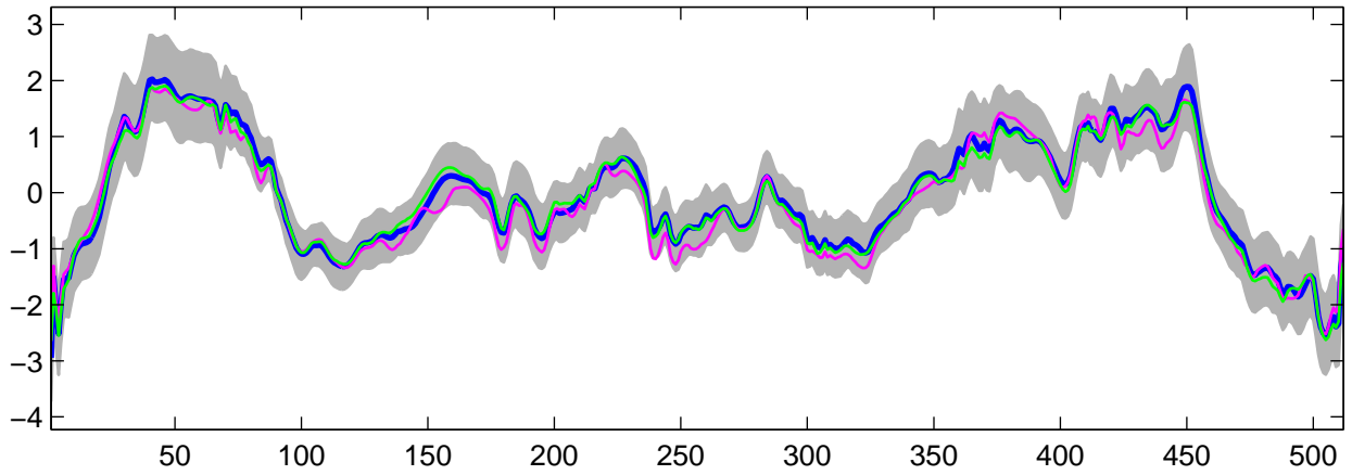
Estimated U_{10}(t) using G-WFMM: t_3 data, run 3
