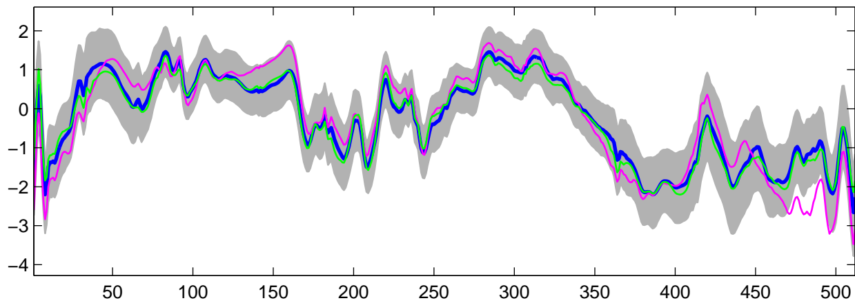
Estimated U_{11}(t) using G-WFMM: DE data, run 3
