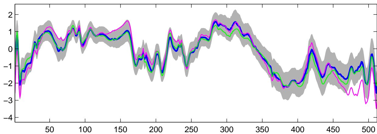
Estimated U_{11}(t) using R-WFMM: DE data, run 3
