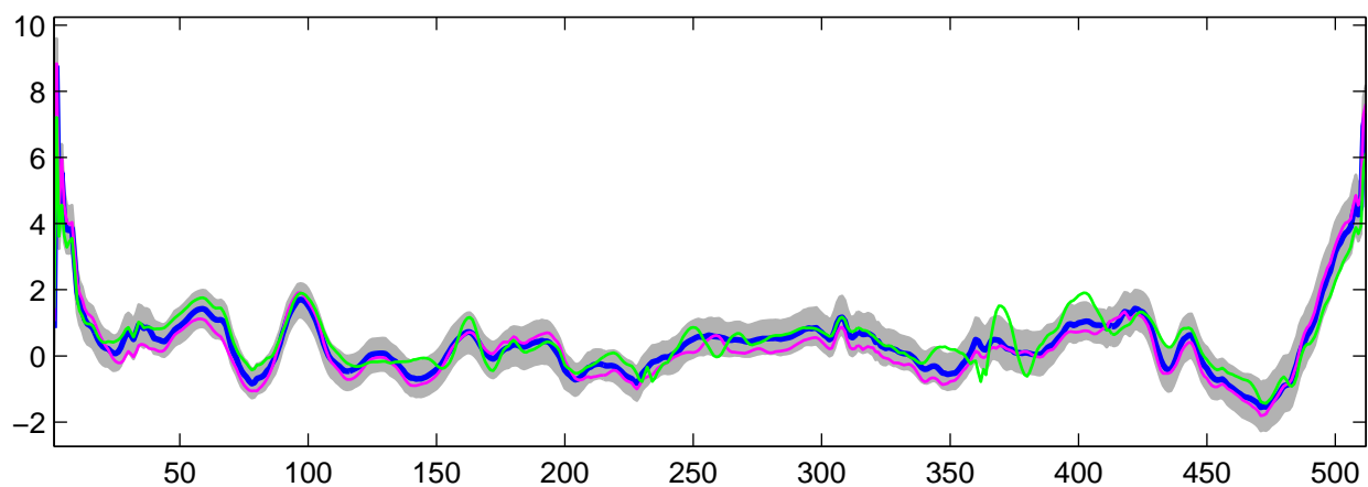
Estimated U_{11}(t) using R-WFMM: t_2 data, run 3
