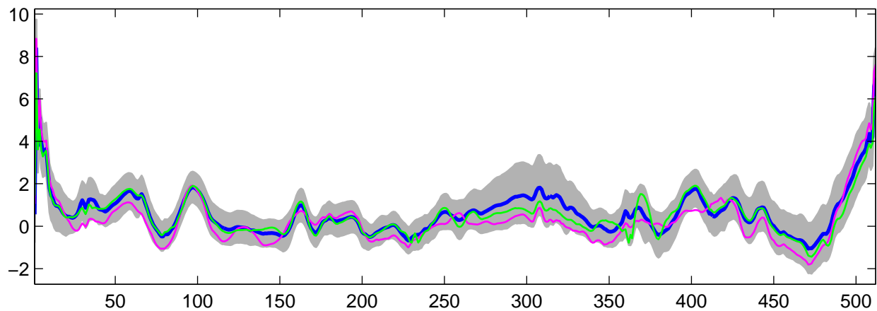
Estimated U_{11}(t) using G-WFMM: t_2 data, run 3
