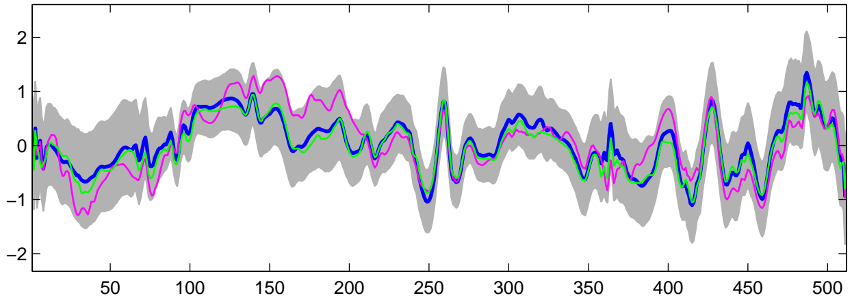
Estimated U_{11}(t) using G-WFMM: t_3 data, run 3
