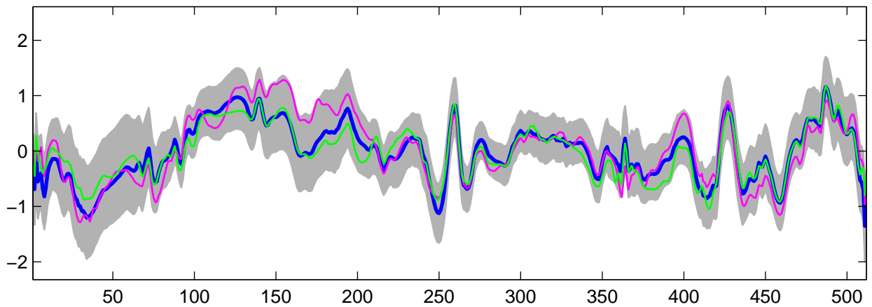
Estimated U_{11}(t) using R-WFMM: t_3 data, run 3
