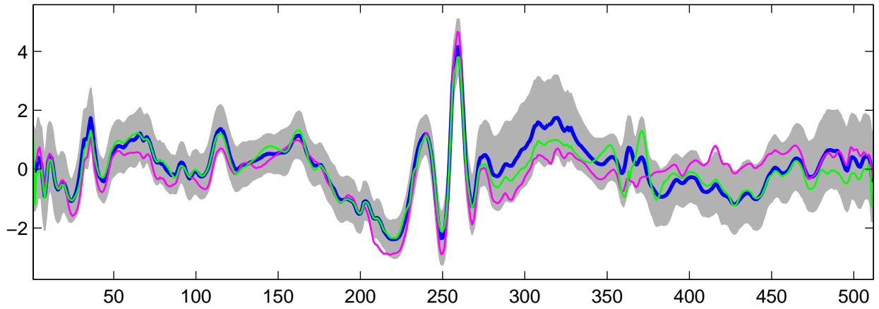
Estimated U_{12}(t) using G-WFMM: t_2 data, run 3
