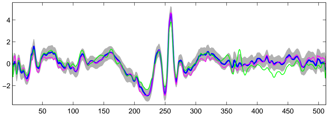
Estimated U_{12}(t) using R-WFMM: t_2 data, run 3
