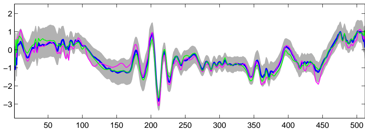
Estimated U_{12}(t) using R-WFMM: t_3 data, run 3
