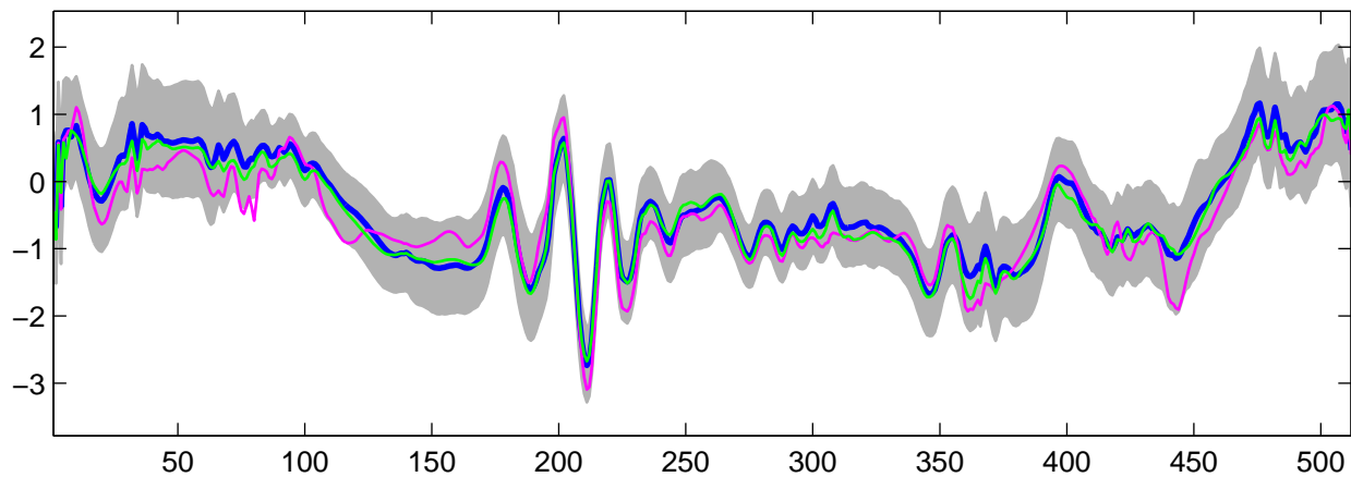
Estimated U_{12}(t) using G-WFMM: t_3 data, run 3
