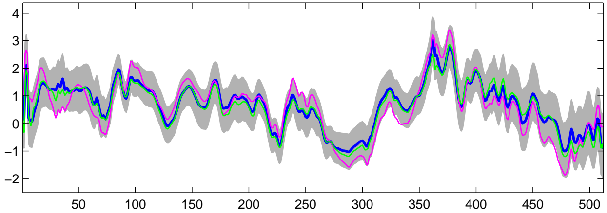
Estimated U_{13}(t) using G-WFMM: Normal data, run 3
