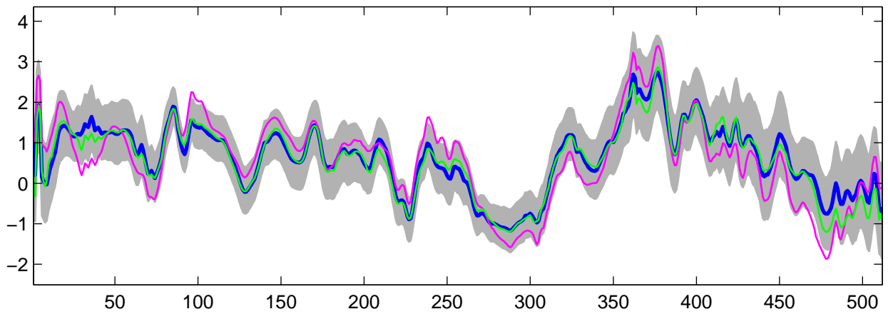
Estimated U_{13}(t) using R-WFMM: Normal data, run 3
