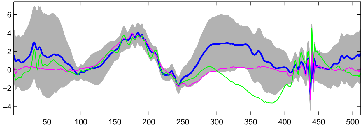
Estimated U_{13}(t) using G-WFMM: t_1 data, run 3
