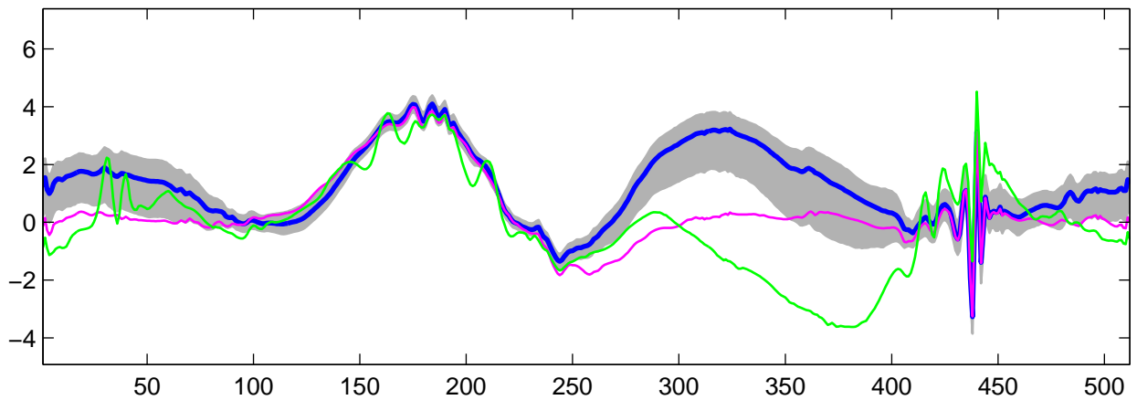
Estimated U_{13}(t) using R-WFMM: t_1 data, run 3
