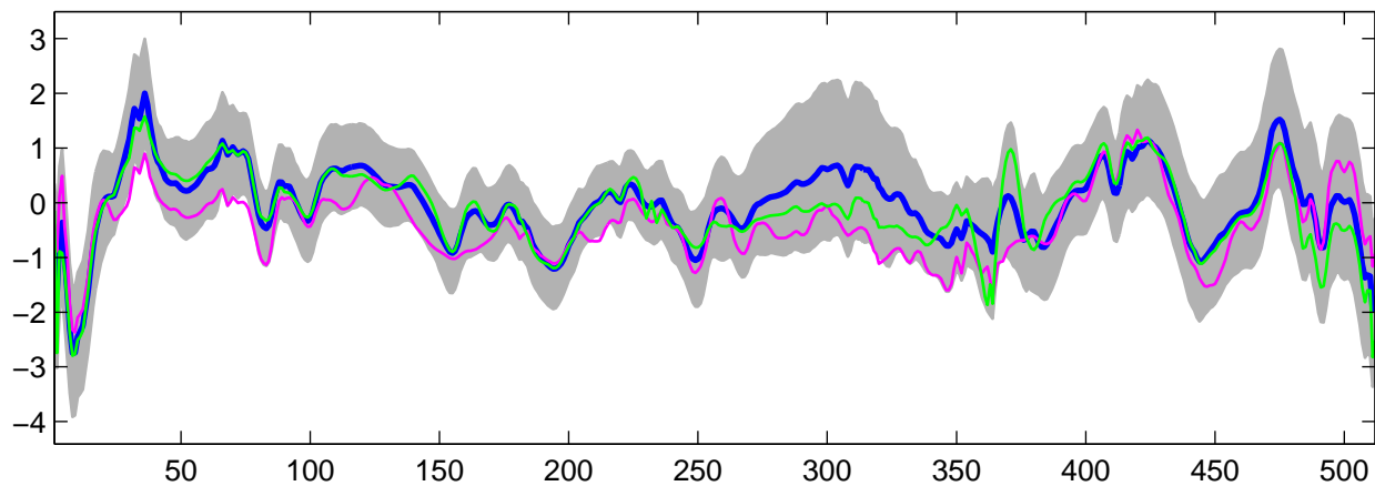
Estimated U_{13}(t) using G-WFMM: t_2 data, run 3
