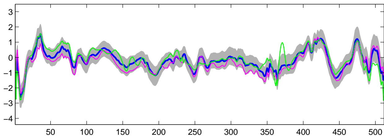
Estimated U_{13}(t) using R-WFMM: t_2 data, run 3
