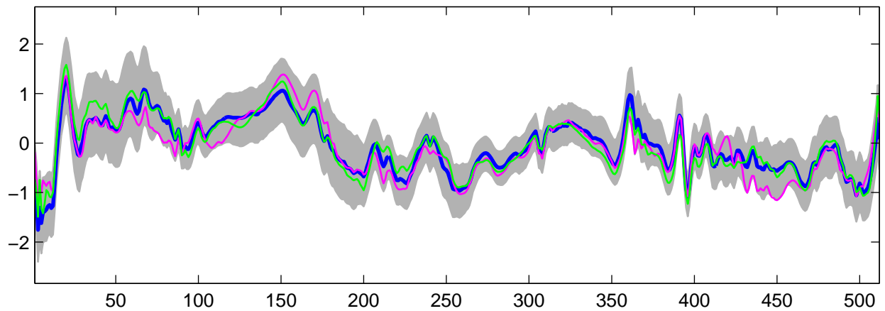
Estimated U_{13}(t) using R-WFMM: t_3 data, run 3
