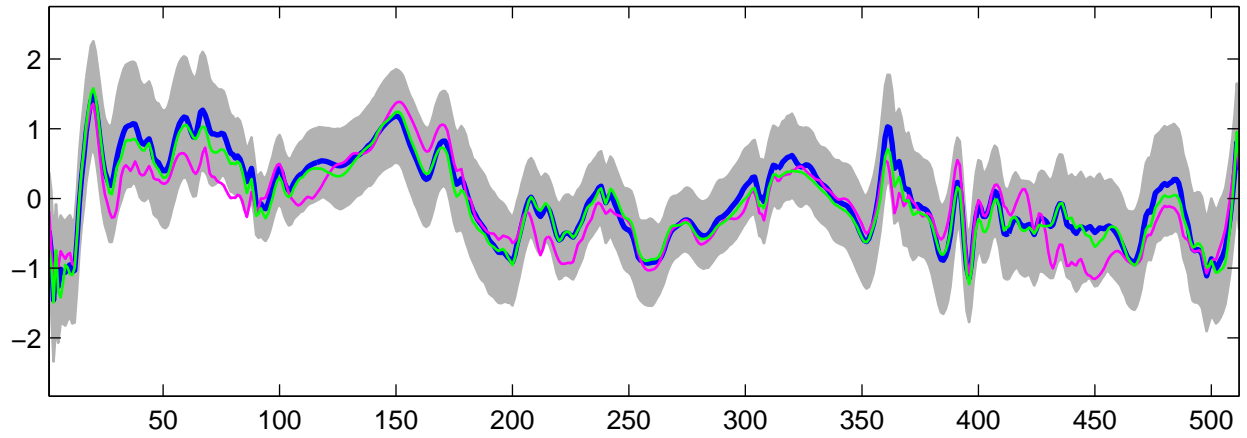
Estimated U_{13}(t) using G-WFMM: t_3 data, run 3
