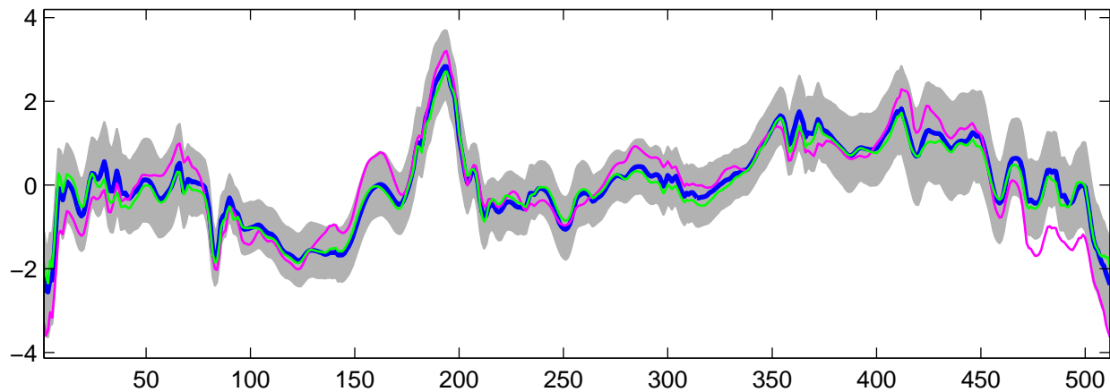
Estimated U_{14}(t) using G-WFMM: DE data, run 3
