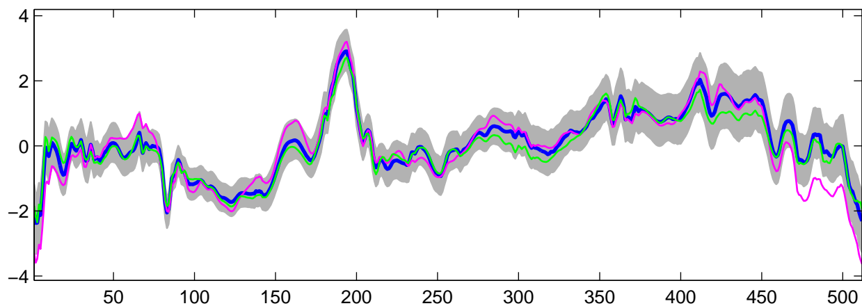
Estimated U_{14}(t) using R-WFMM: DE data, run 3
