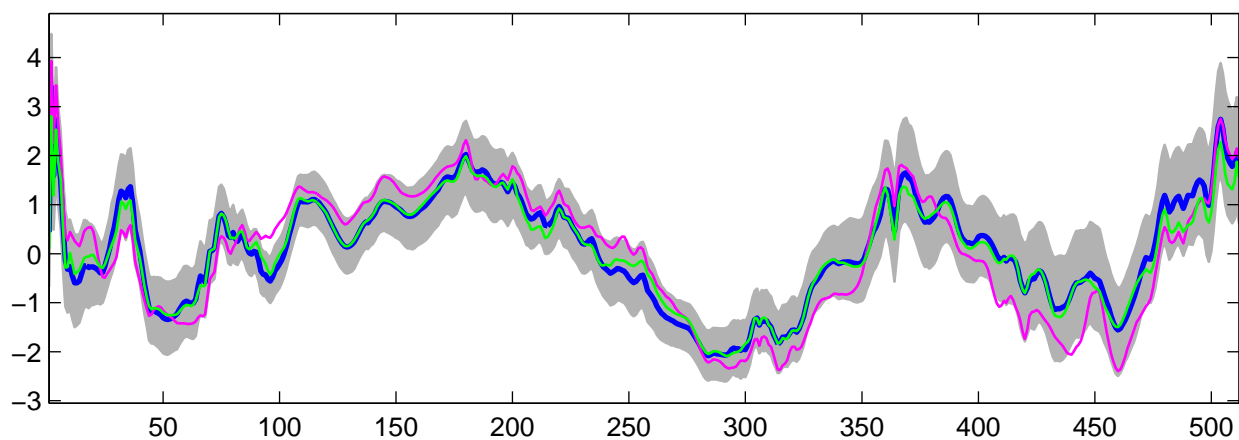
Estimated U_{14}(t) using R-WFMM: Normal data, run 3
