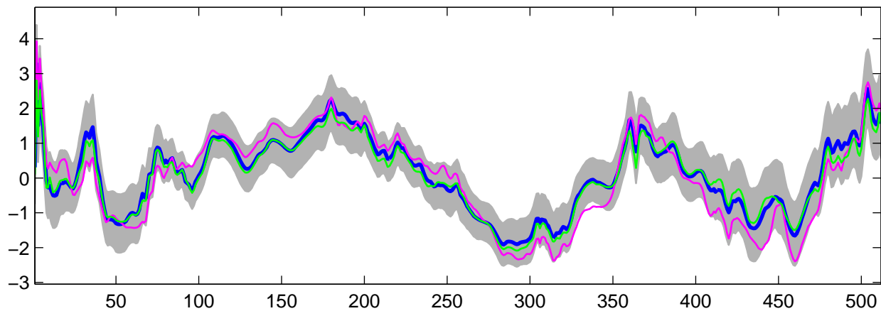
Estimated U_{14}(t) using G-WFMM: Normal data, run 3
