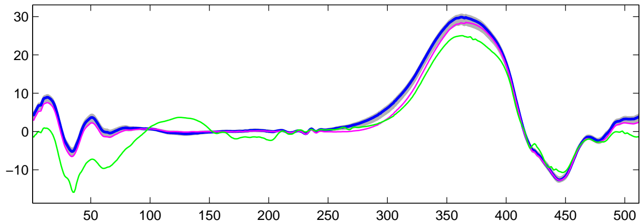
Estimated U_{14}(t) using R-WFMM: t_1 data, run 3
