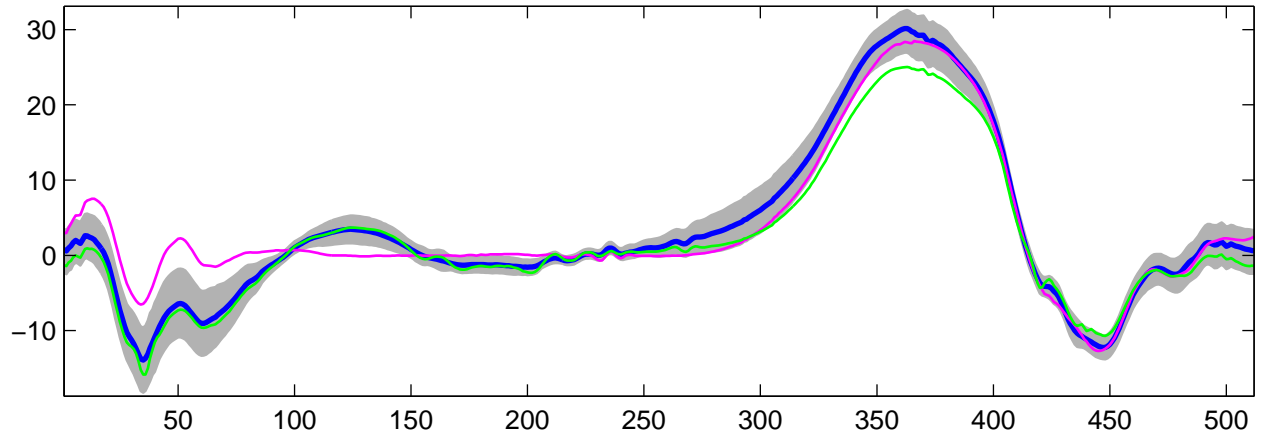
Estimated U_{14}(t) using G-WFMM: t_1 data, run 3
