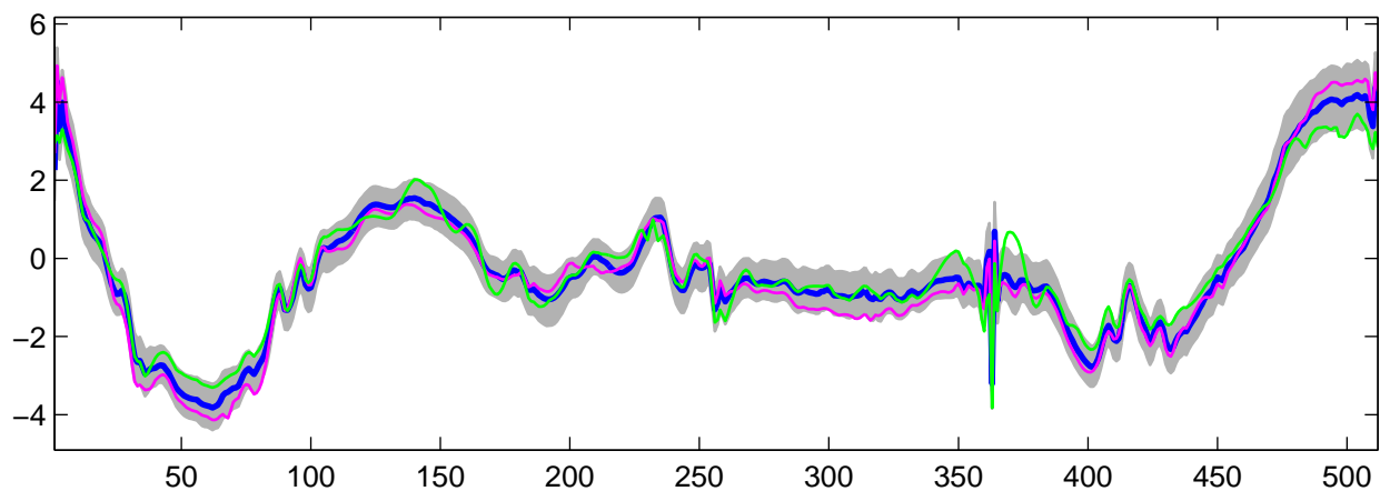
Estimated U_{15}(t) using R-WFMM: t_2 data, run 3
