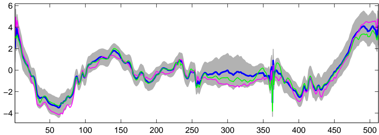
Estimated U_{15}(t) using G-WFMM: t_2 data, run 3
