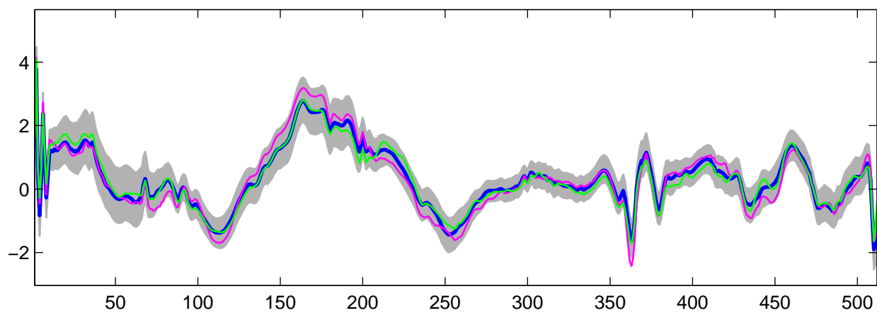
Estimated U_{15}(t) using R-WFMM: t_3 data, run 3
