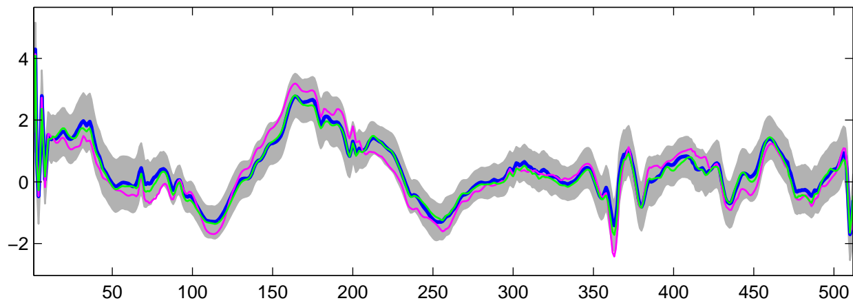
Estimated U_{15}(t) using G-WFMM: t_3 data, run 3
