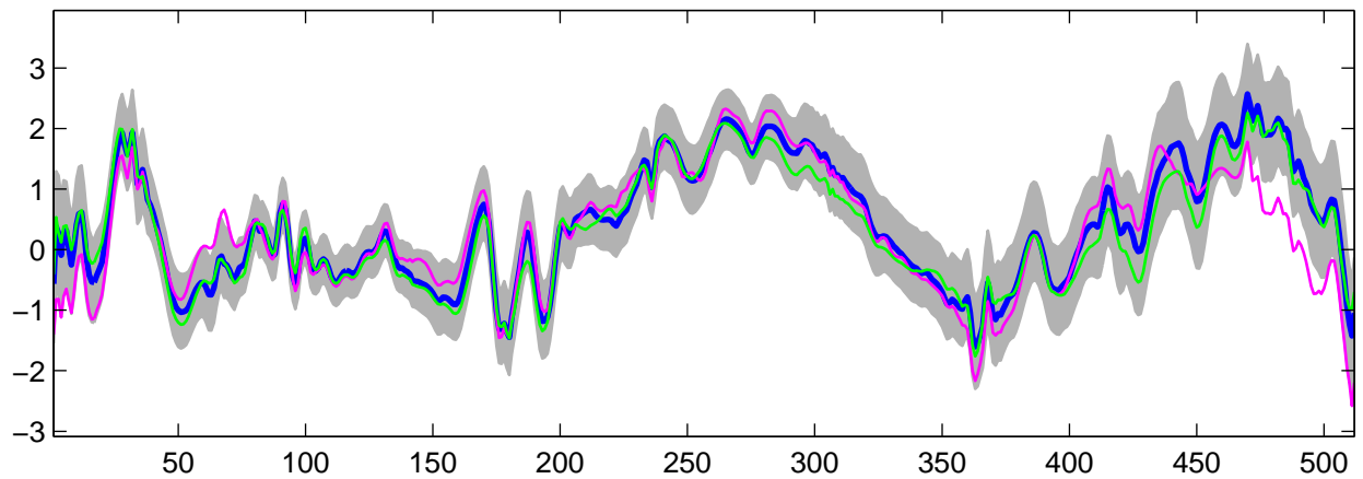
Estimated U_{16}(t) using R-WFMM: DE data, run 3
