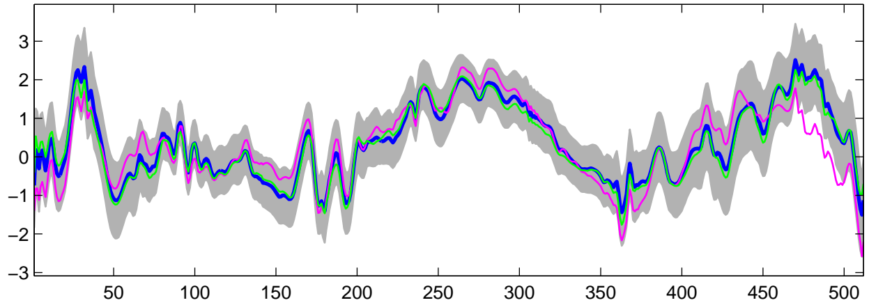
Estimated U_{16}(t) using G-WFMM: DE data, run 3
