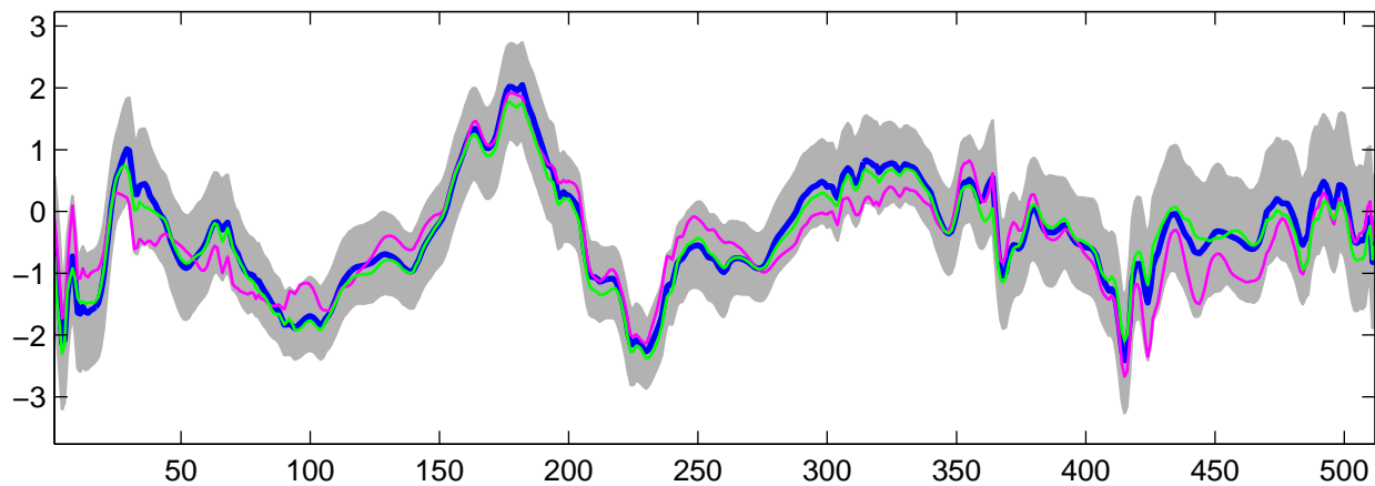
Estimated U_{16}(t) using G-WFMM: Normal data, run 3
