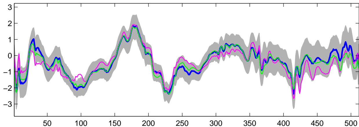
Estimated U_{16}(t) using R-WFMM: Normal data, run 3
