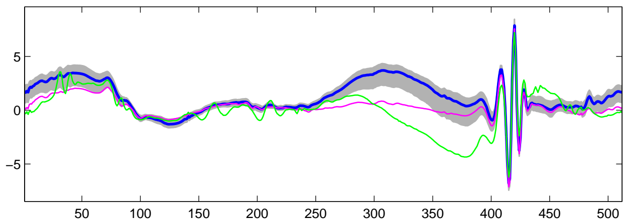
Estimated U_{16}(t) using R-WFMM: t_1 data, run 3
