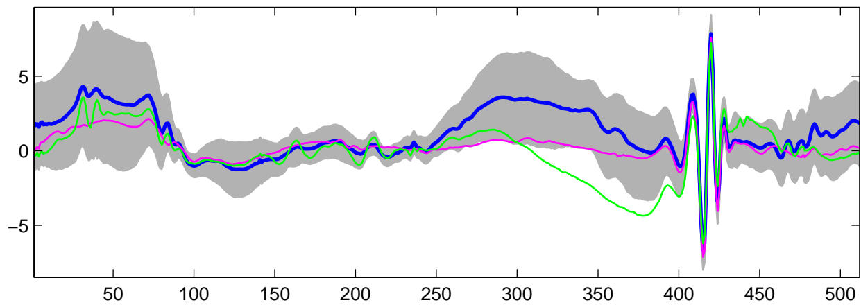
Estimated U_{16}(t) using G-WFMM: t_1 data, run 3
