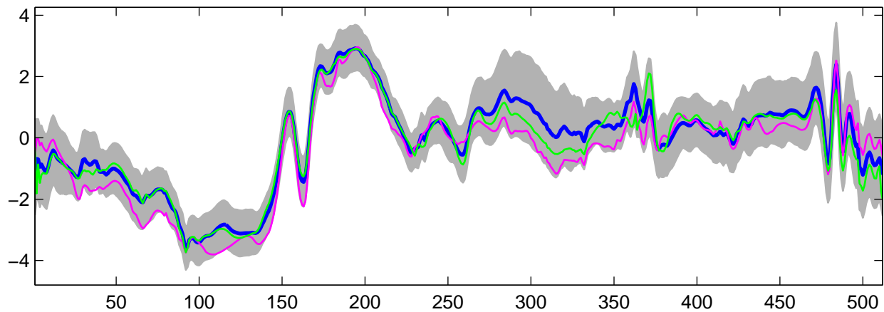
Estimated U_{16}(t) using G-WFMM: t_2 data, run 3
