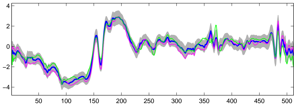
Estimated U_{16}(t) using R-WFMM: t_2 data, run 3
