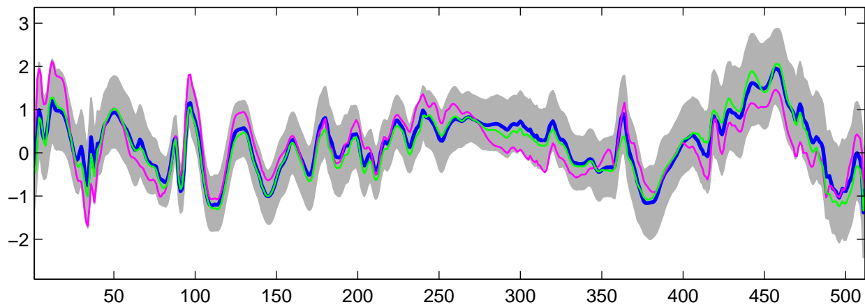
Estimated U_{17}(t) using G-WFMM: Normal data, run 3
