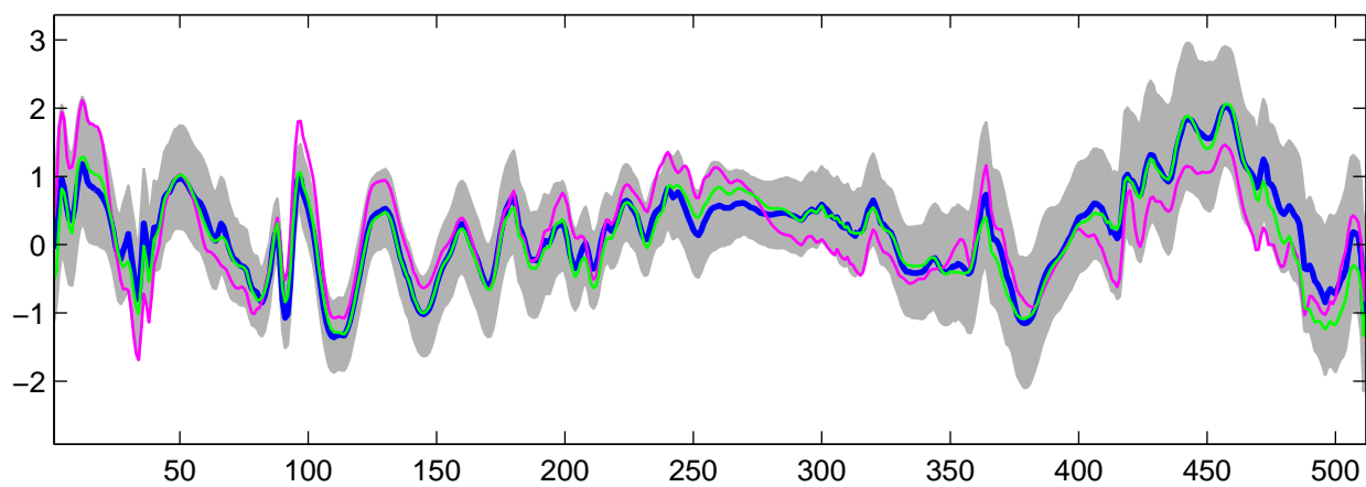
Estimated U_{17}(t) using R-WFMM: Normal data, run 3
