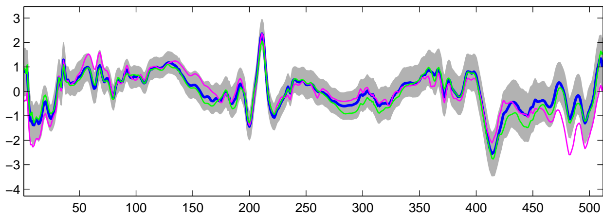
Estimated U_{18}(t) using R-WFMM: DE data, run 3
