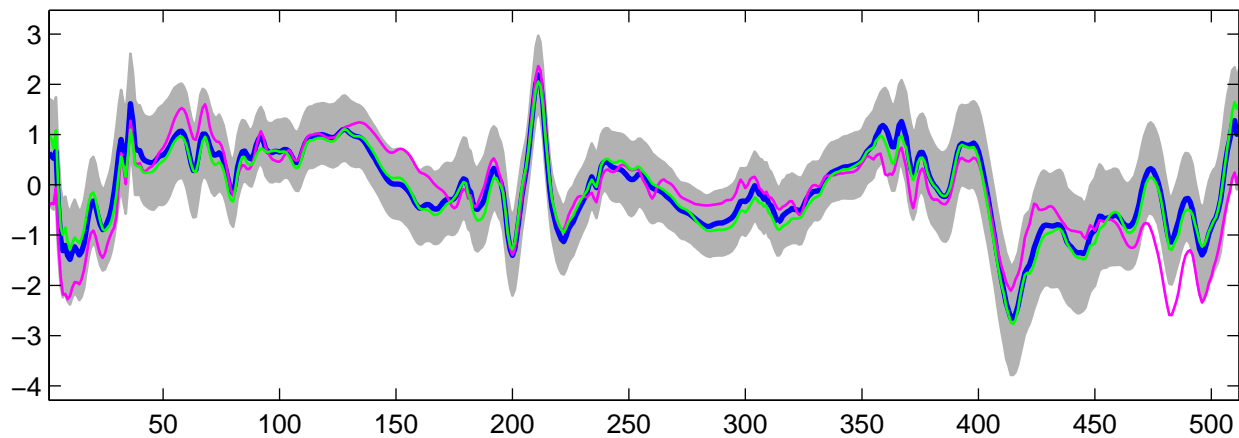
Estimated U_{18}(t) using G-WFMM: DE data, run 3
