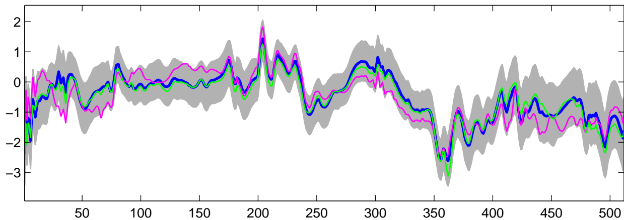
Estimated U_{18}(t) using G-WFMM: Normal data, run 3
