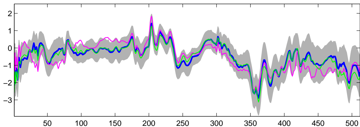
Estimated U_{18}(t) using R-WFMM: Normal data, run 3
