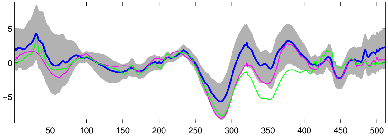
Estimated U_{18}(t) using G-WFMM: t_1 data, run 3
