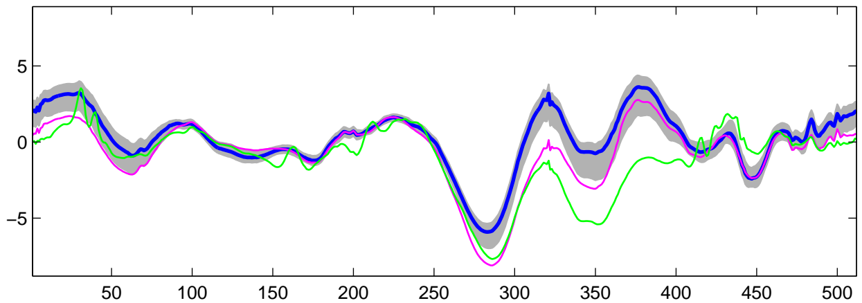
Estimated U_{18}(t) using R-WFMM: t_1 data, run 3
