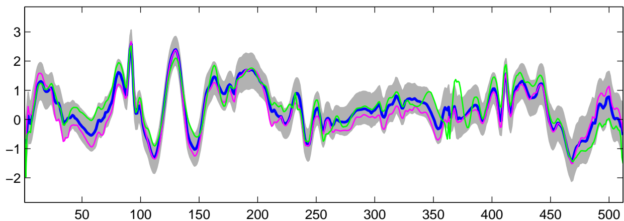
Estimated U_{18}(t) using R-WFMM: t_2 data, run 3
