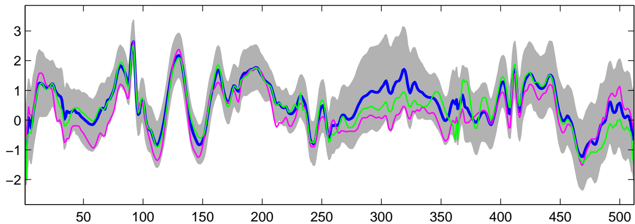
Estimated U_{18}(t) using G-WFMM: t_2 data, run 3
