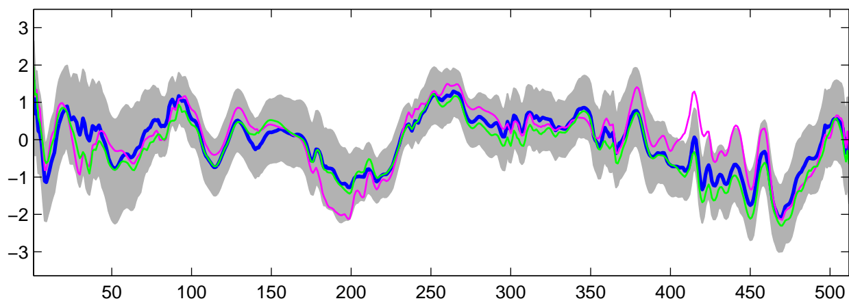
Estimated U_{19}(t) using R-WFMM: Normal data, run 3
