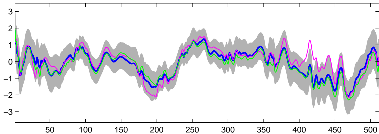
Estimated U_{19}(t) using G-WFMM: Normal data, run 3
