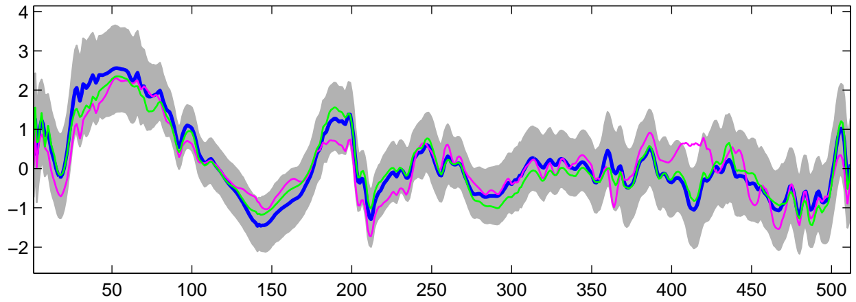
Estimated U_{20}(t) using G-WFMM: DE data, run 3
