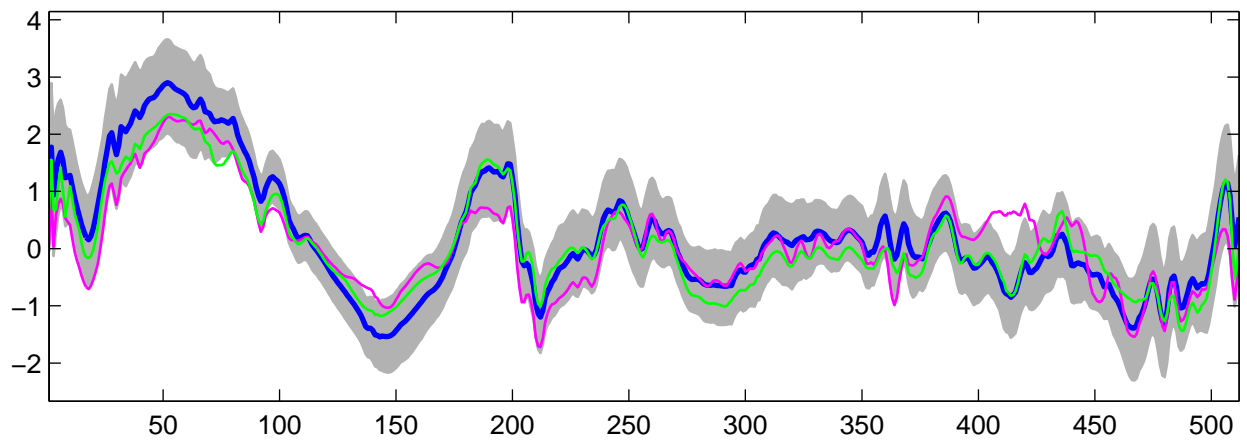
Estimated U_{20}(t) using R-WFMM: DE data, run 3
