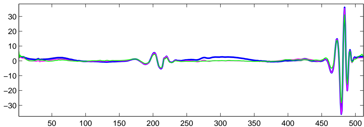
Estimated U_{20}(t) using R-WFMM: t_1 data, run 3
