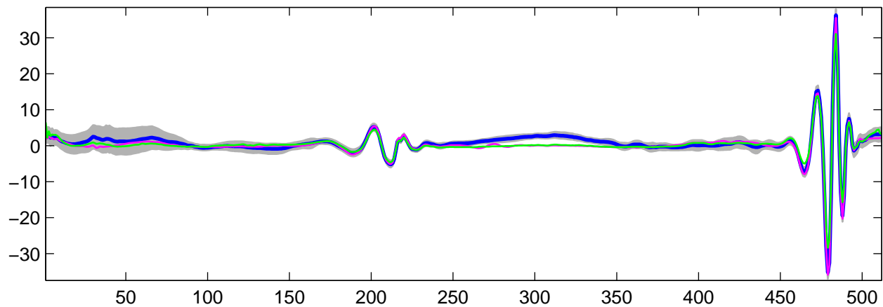
Estimated U_{20}(t) using G-WFMM: t_1 data, run 3
