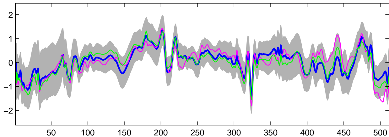
Estimated U_{20}(t) using G-WFMM: t_3 data, run 3
