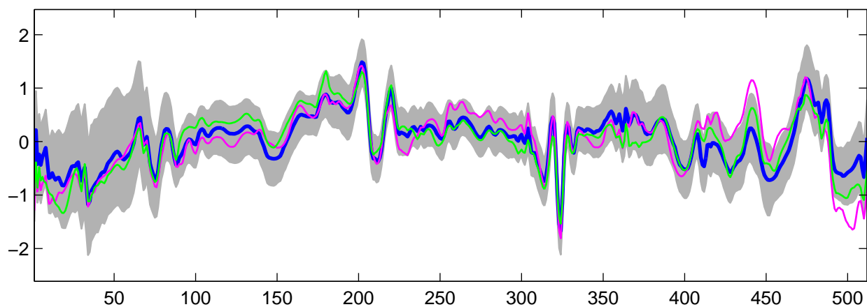
Estimated U_{20}(t) using R-WFMM: t_3 data, run 3
