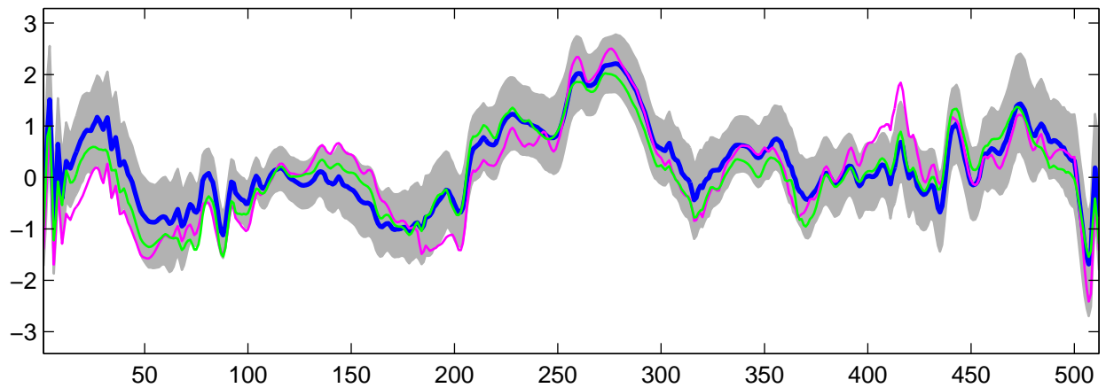
Estimated U_{21}(t) using R-WFMM: DE data, run 3
