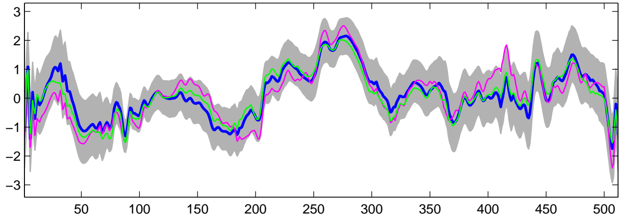
Estimated U_{21}(t) using G-WFMM: DE data, run 3
