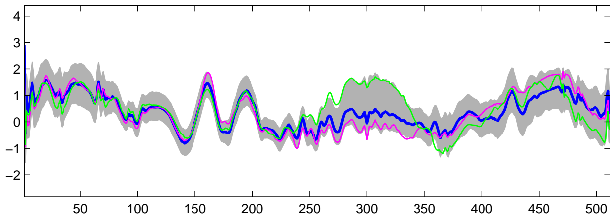
Estimated U_{21}(t) using R-WFMM: t_2 data, run 3
