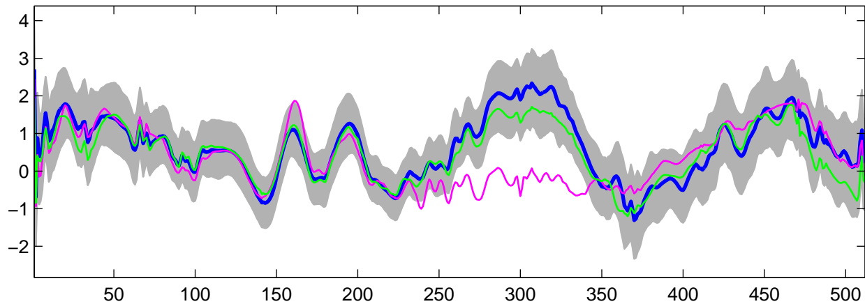
Estimated U_{21}(t) using G-WFMM: t_2 data, run 3
