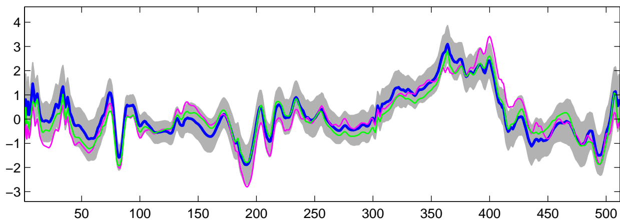
Estimated U_{22}(t) using R-WFMM: DE data, run 3
