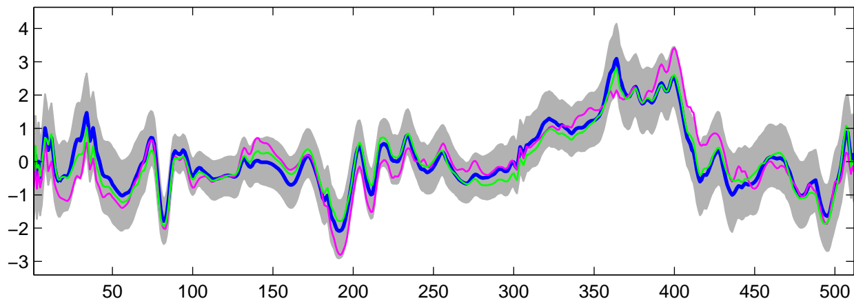
Estimated U_{22}(t) using G-WFMM: DE data, run 3
