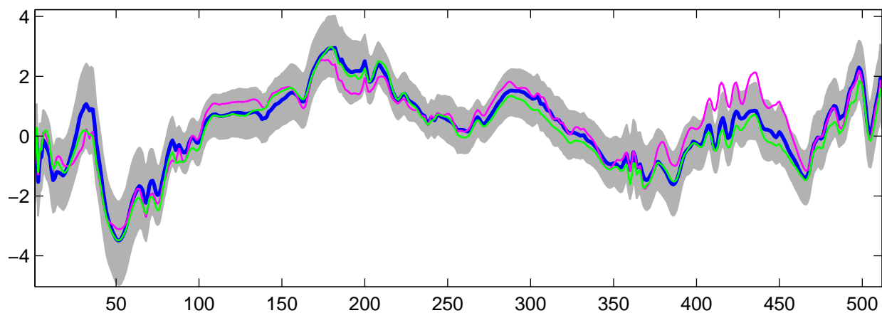
Estimated U_{22}(t) using R-WFMM: Normal data, run 3
