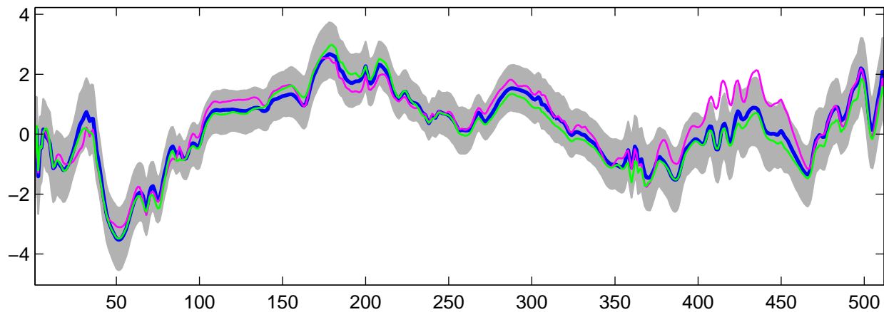
Estimated U_{22}(t) using G-WFMM: Normal data, run 3
