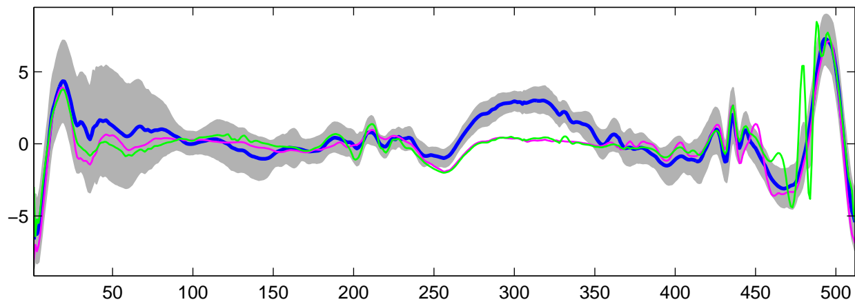
Estimated U_{22}(t) using G-WFMM: t_1 data, run 3
