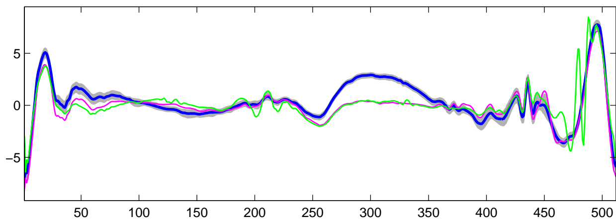
Estimated U_{22}(t) using R-WFMM: t_1 data, run 3
