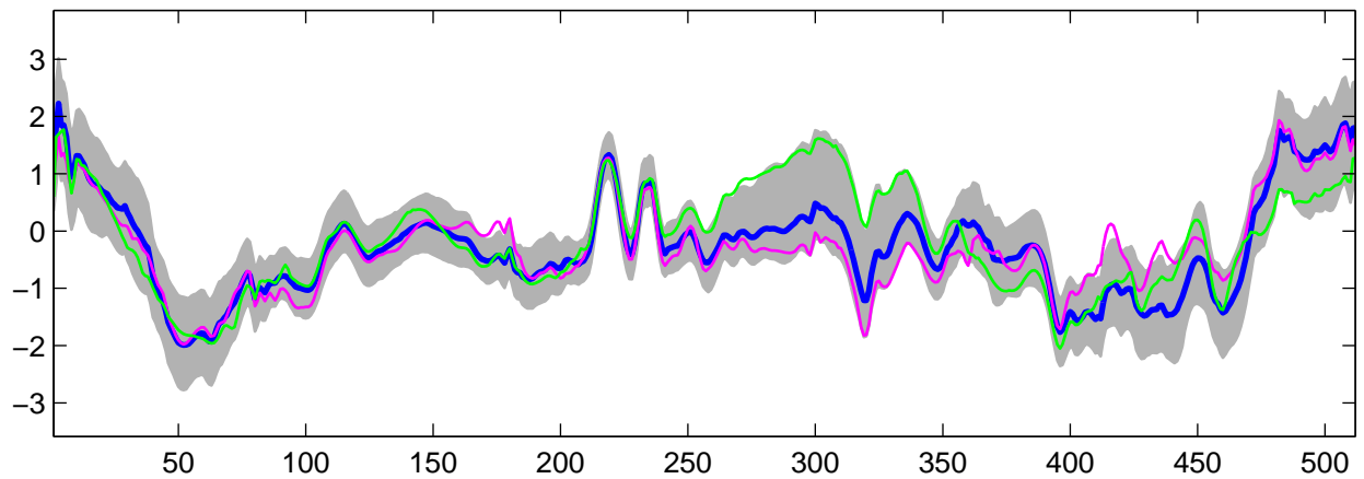
Estimated U_{22}(t) using R-WFMM: t_2 data, run 3
