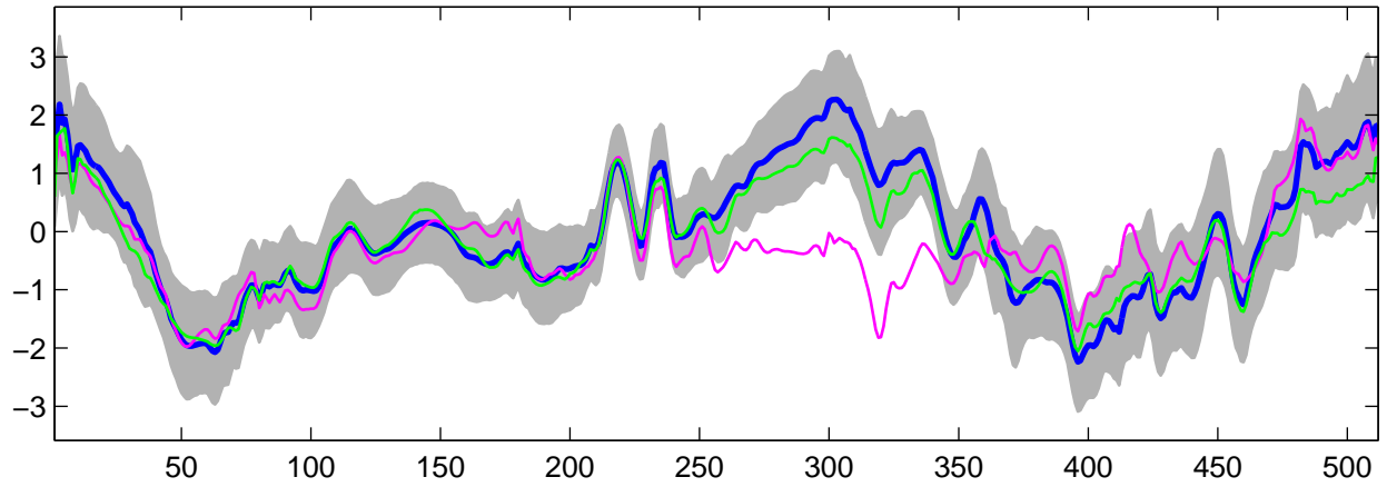
Estimated U_{22}(t) using G-WFMM: t_2 data, run 3
